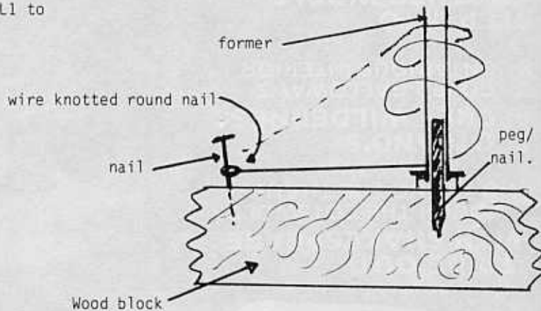
Winding Jig
